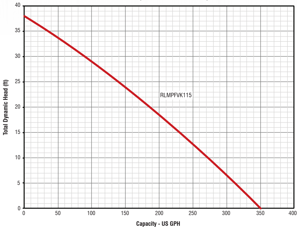
Multi-Purpose Transfer Pump
